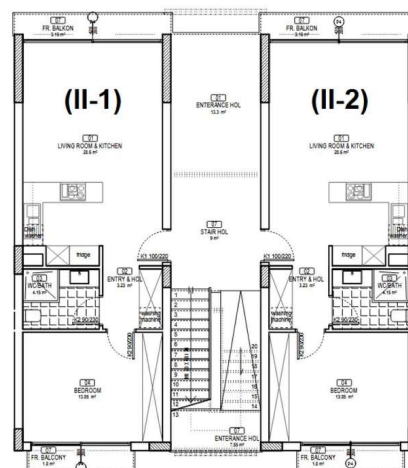
TYPE II GROUND FLOOR PLAN(1+1)
